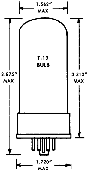
OUTLINE DRAWING
