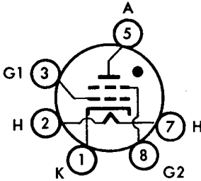
BASING DIAGRAM BOTTOM VIEW 6C0
